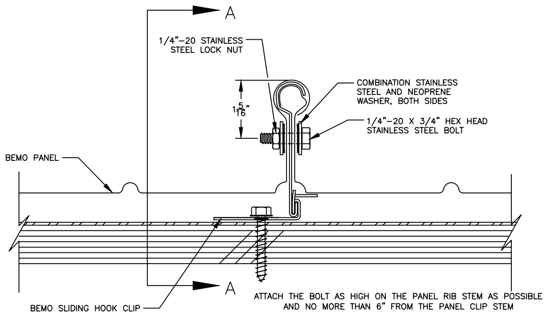
BEMO DEFLECTION LIMITING BOLT FOR HIGH WIND UPLIFT AREAS
