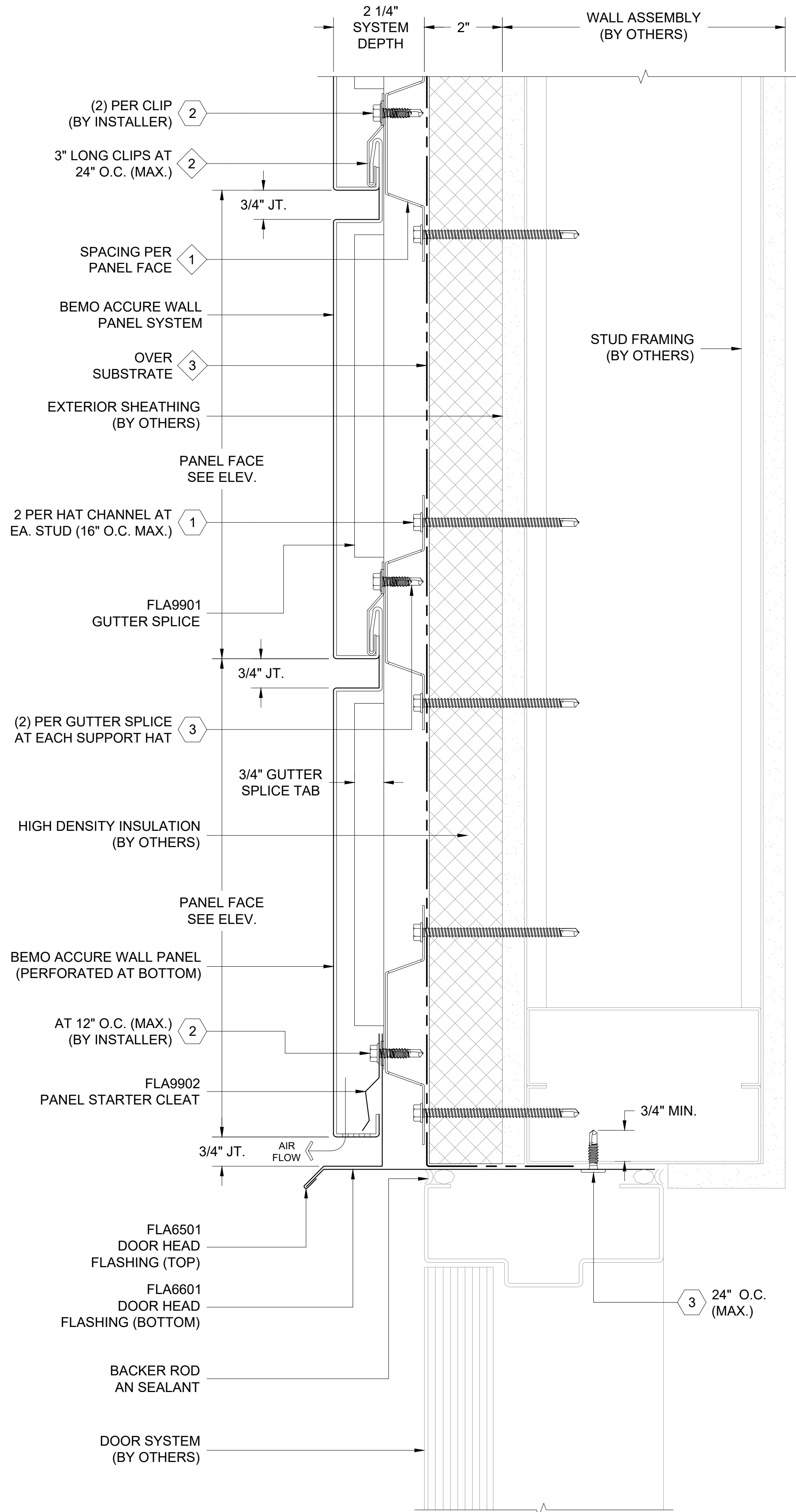
1 DOOR HEAD DETAIL D1 REF. ARCH. DET. -
