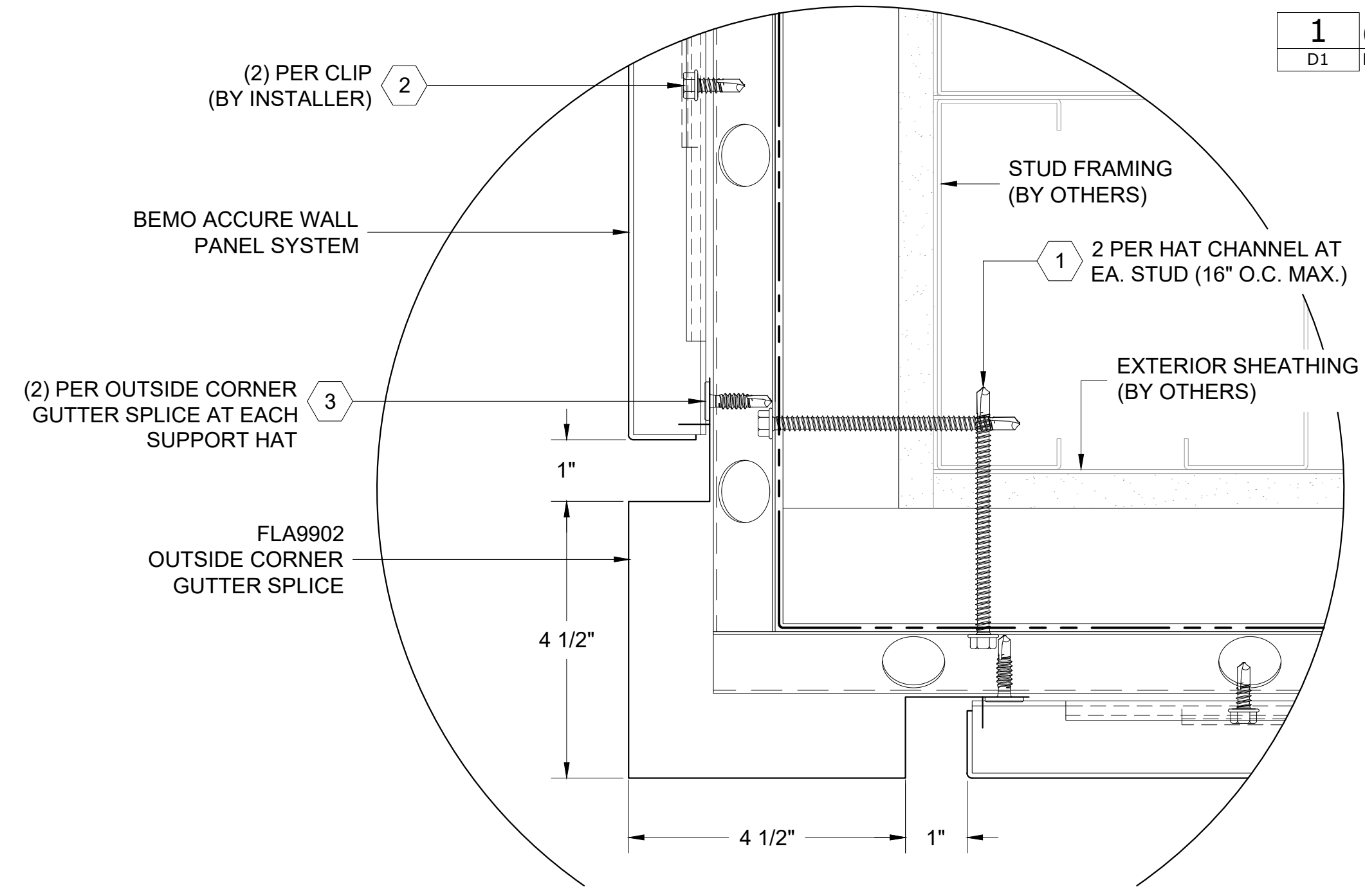
ALTERNATE OUTSIDE CORNER DETAIL W/ TRIM
