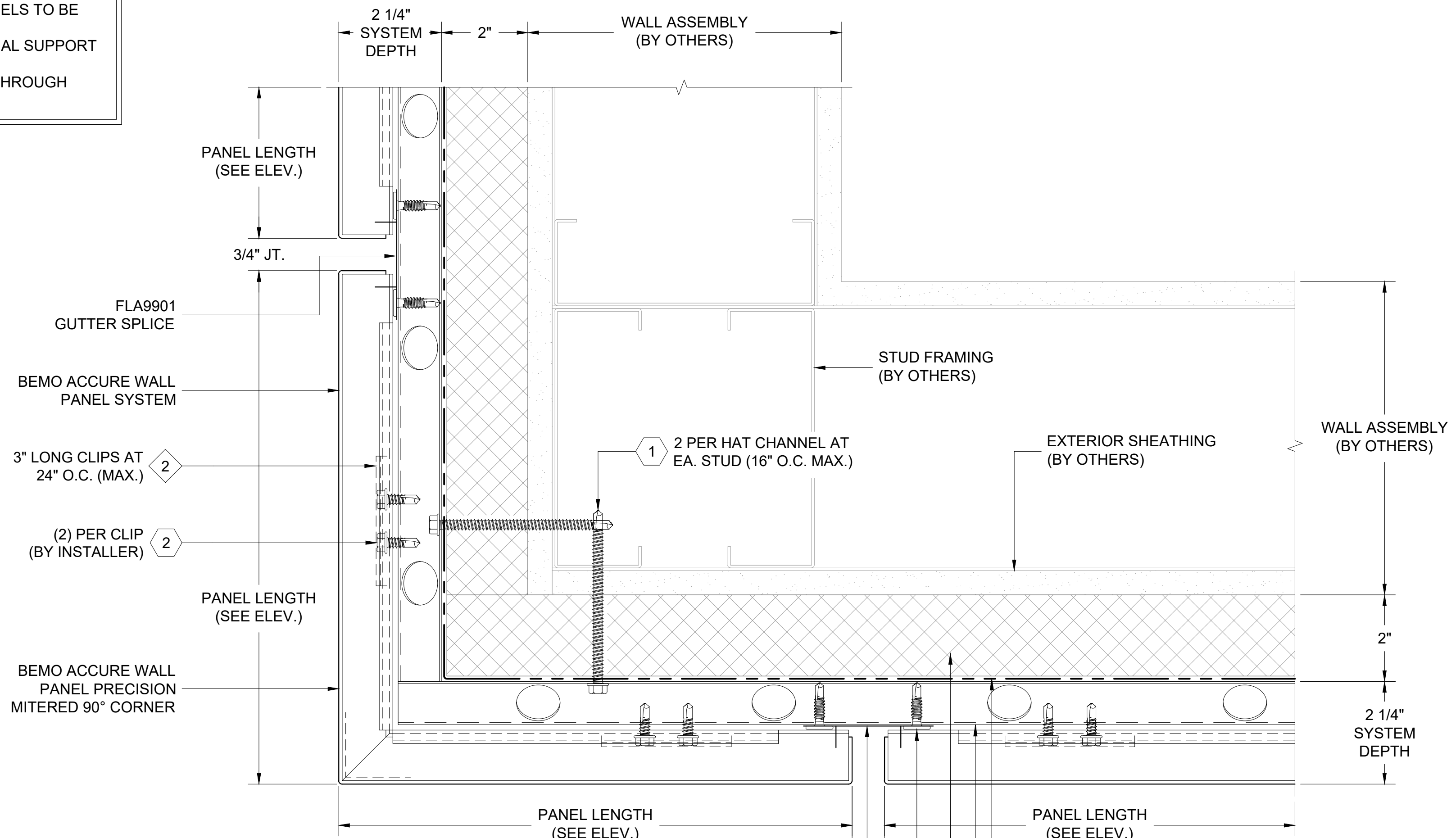
PLAN VIEW
