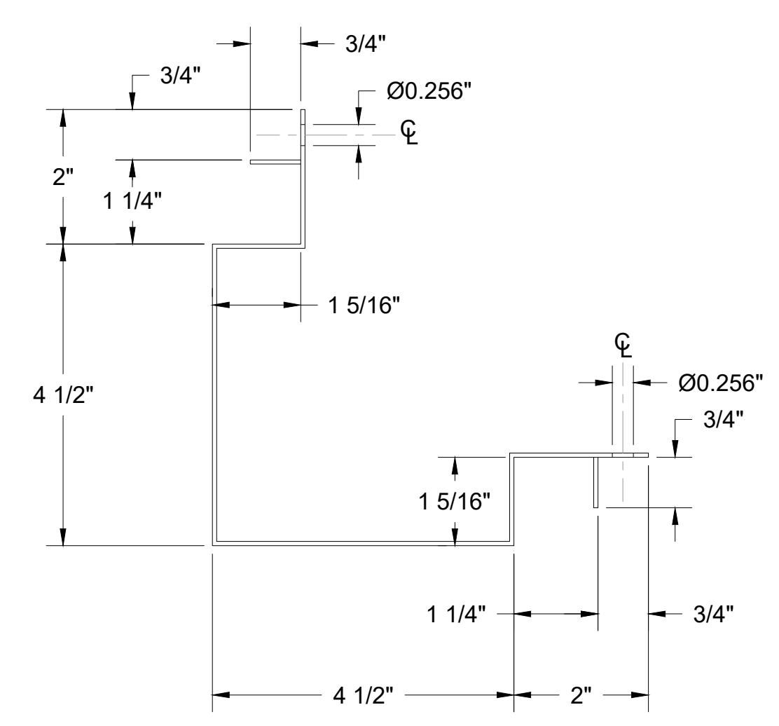
FLA9902 OUTSIDE CORNER GUTTER SPLICE (PROFILE)
