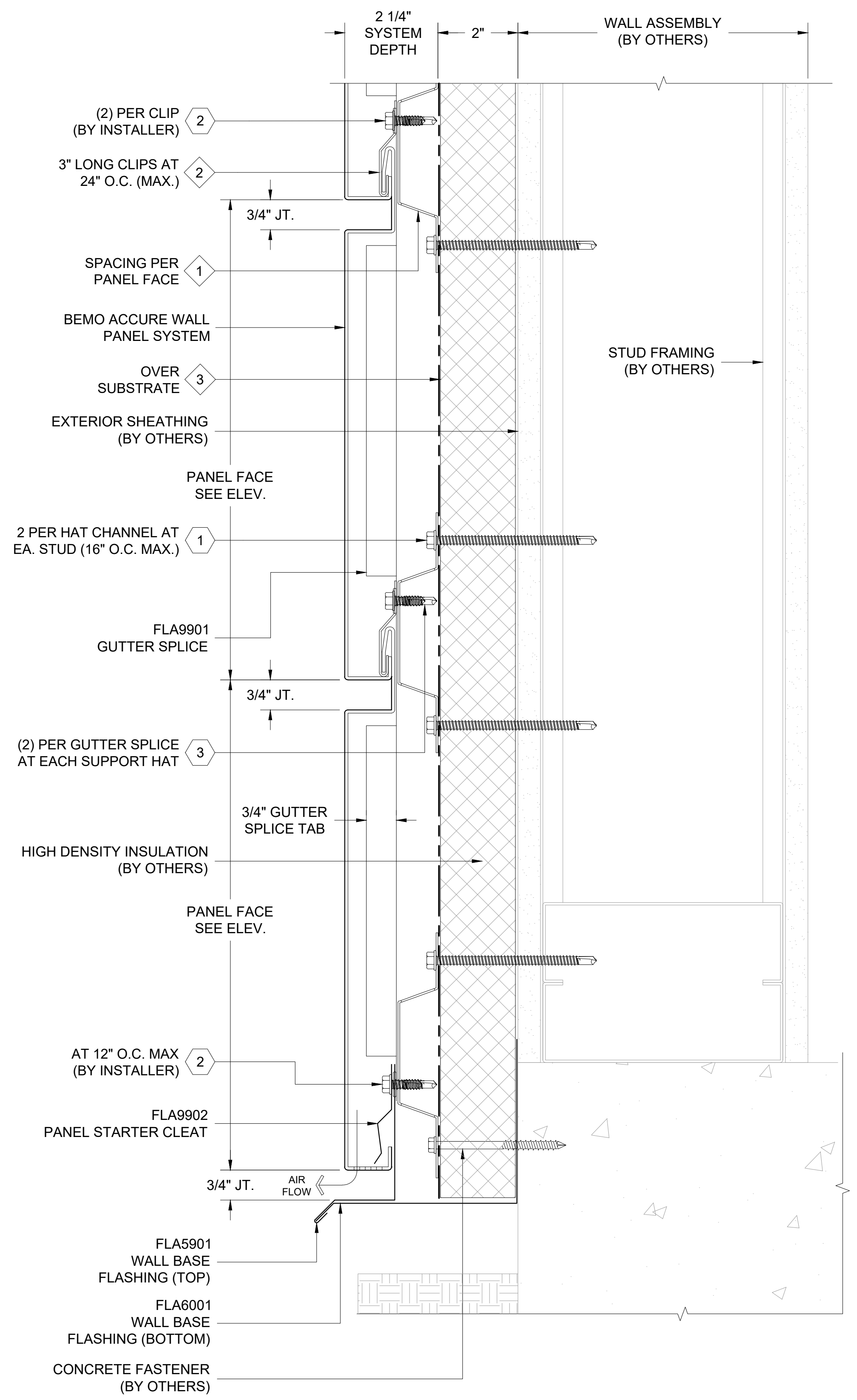
1 WALL BASE AT SLAB DETAIL D1 REF. ARCH. DET. -
