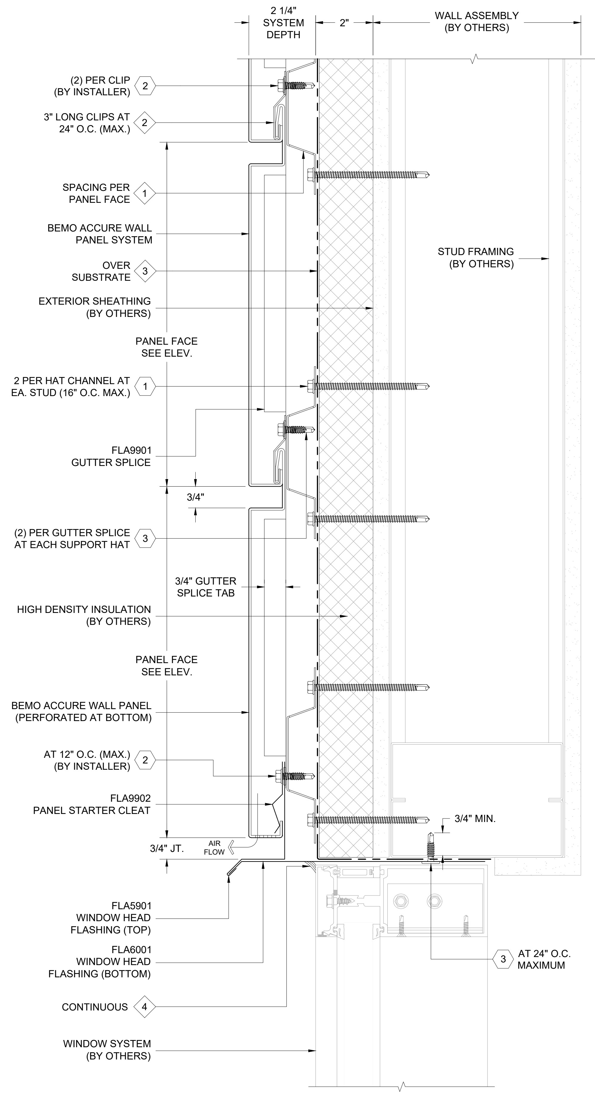
1 WINDOW HEAD DETAIL D1 REF. ARCH. DET. -
