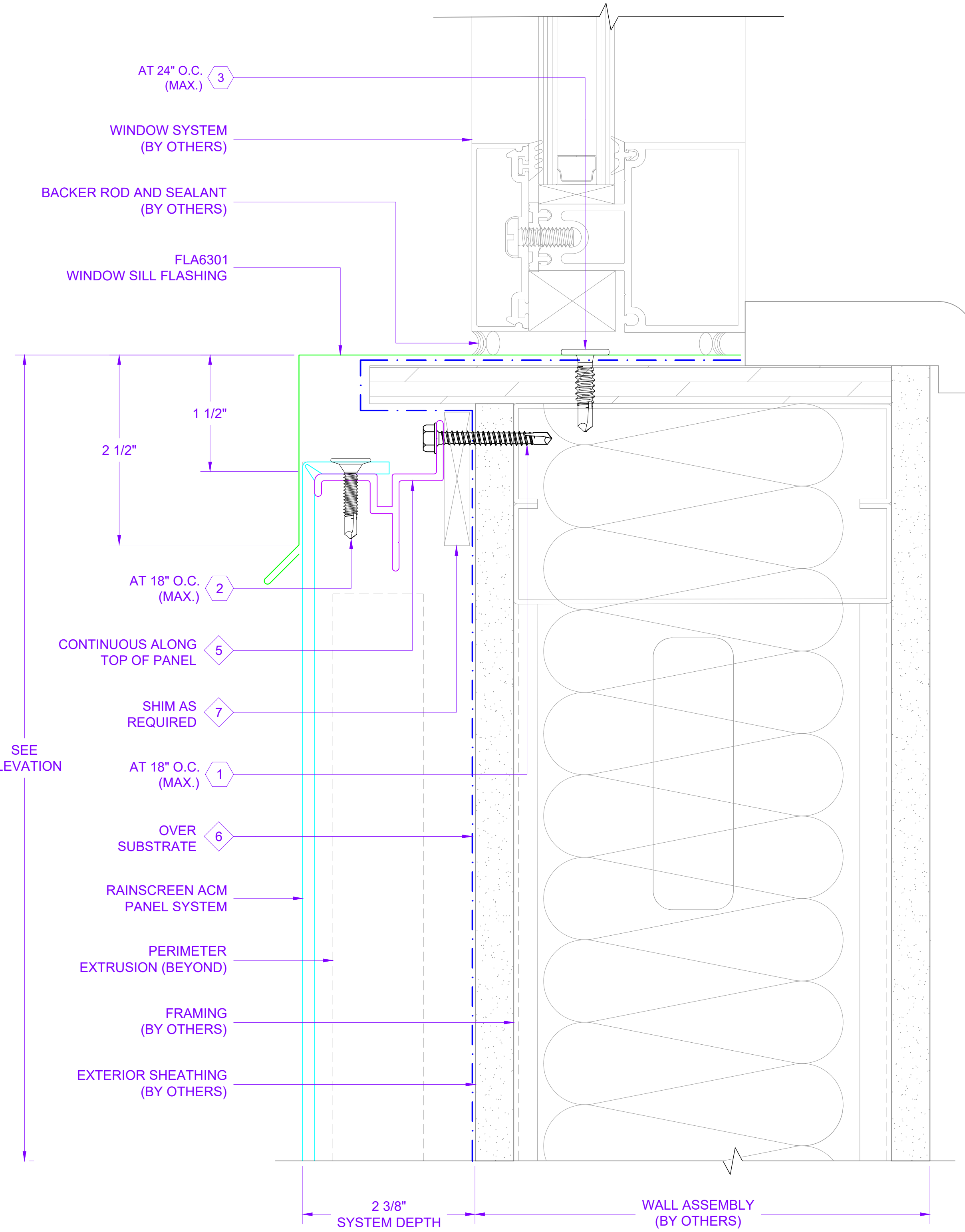
1 WINDOW SILL DETAIL D1 REF. ARCH. DET. -
