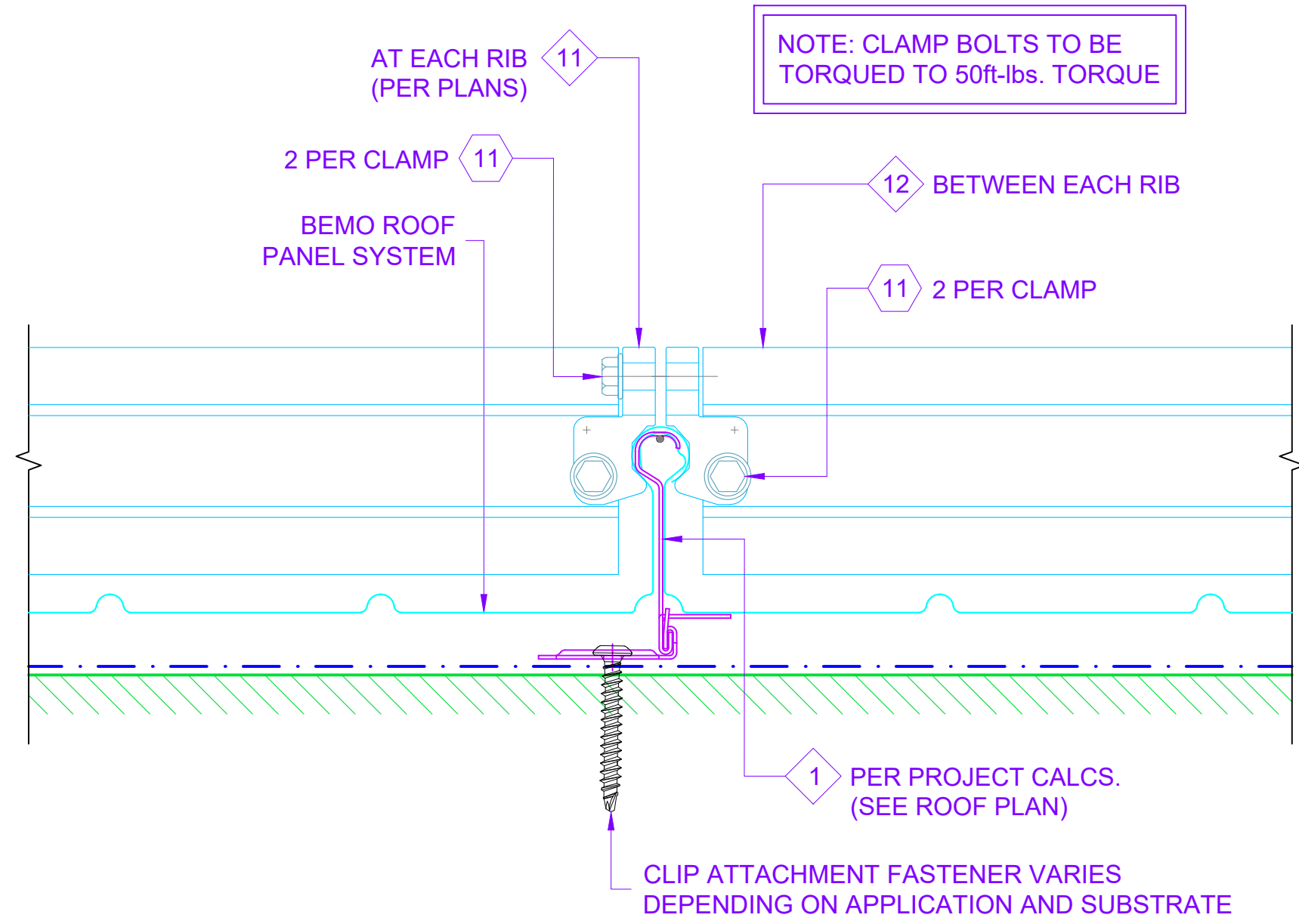
2 SNOW RETENTION DETAIL D1 REF. ARCH. DET. -
