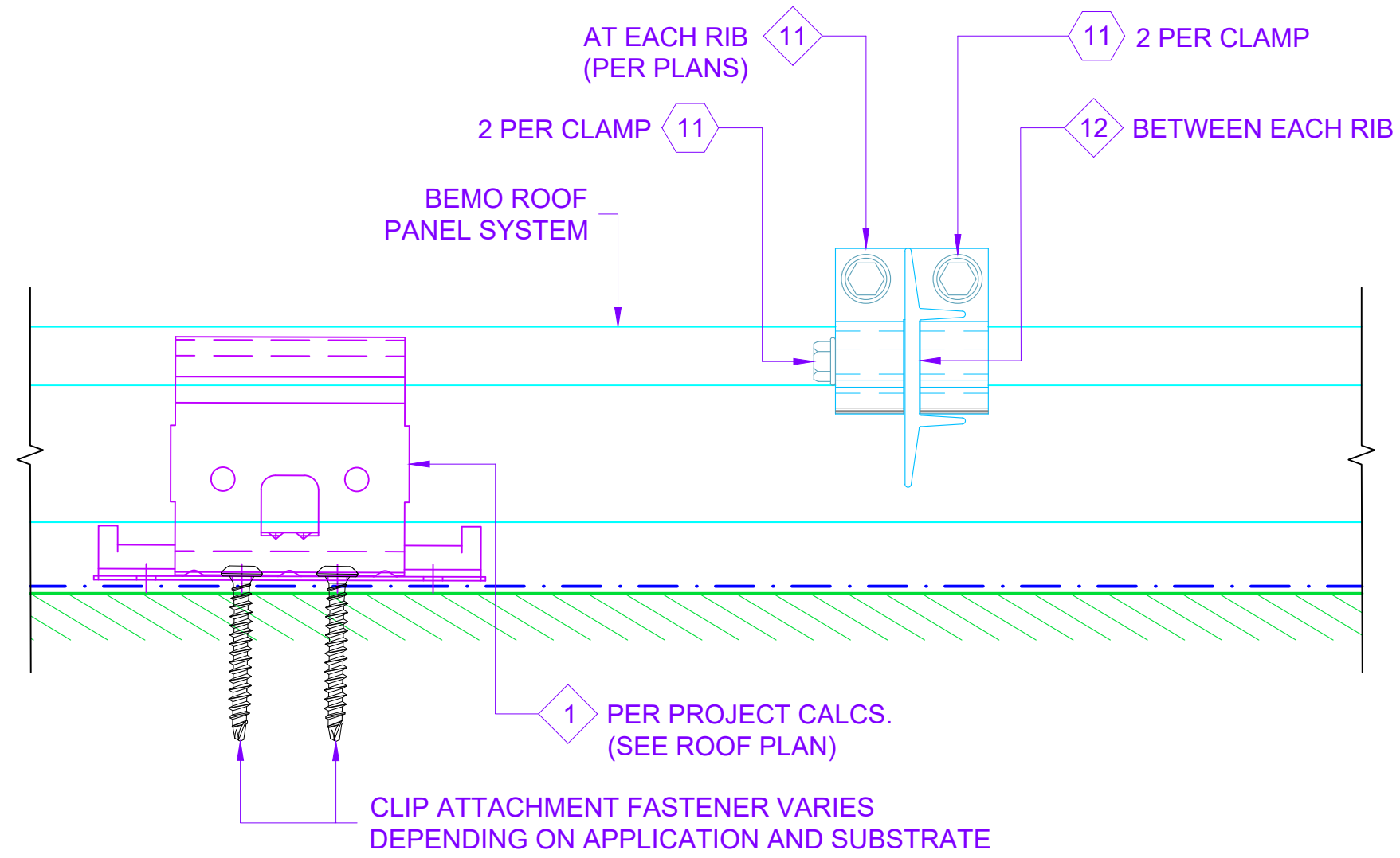
1 SNOW RETENTION DETAIL D1 REF. ARCH. DET. -
