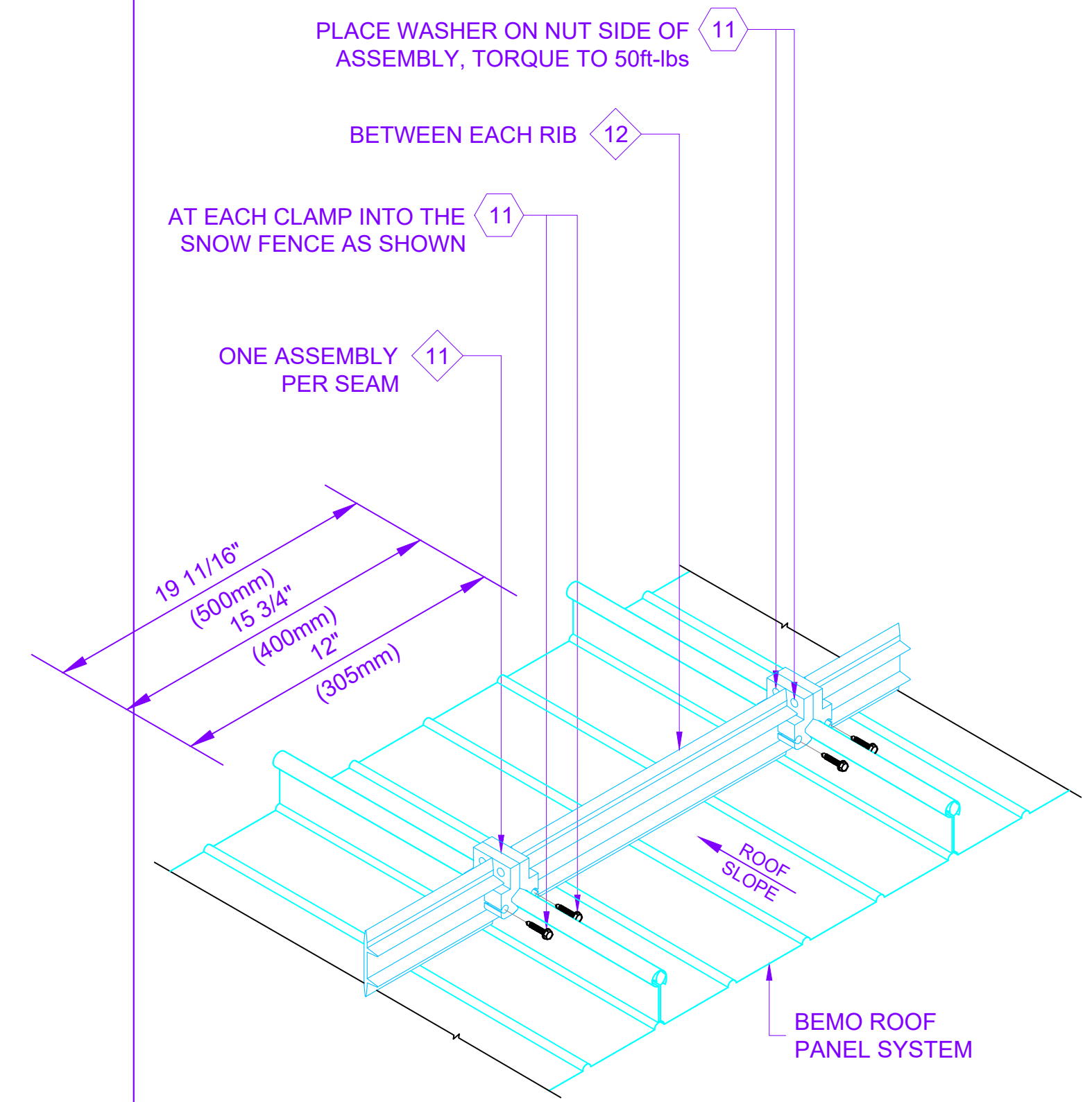
ISOMETRIC VIEW
