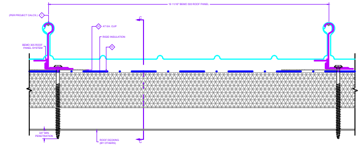
MEMO 500 PANEL 'SLIDING' DETAIL - LOOK CLIP
