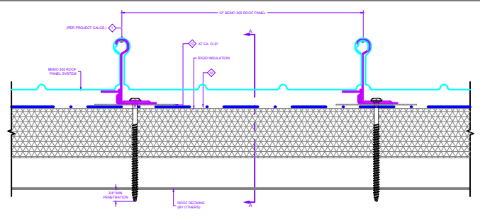
MEMO 305 PANEL 'SLIDING' DETAIL - LOOK CLIP
