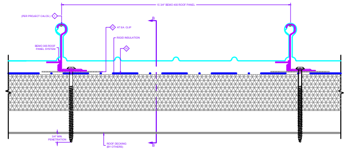
MEMO 400 PANEL 'SLIDING' DETAIL - LOOK CLIP
