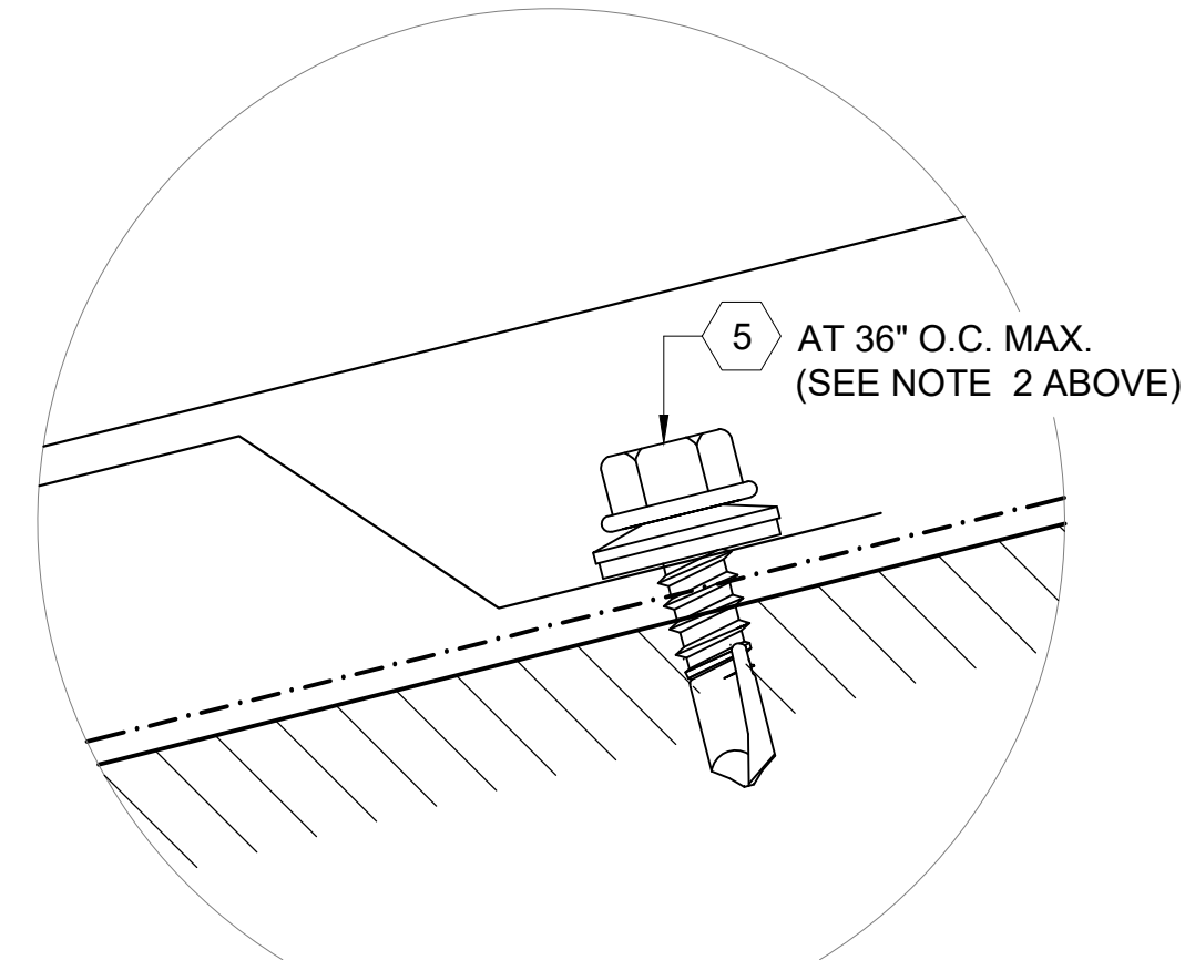
ALTERNATE FASTENING AT FLASHING SUPPORT
