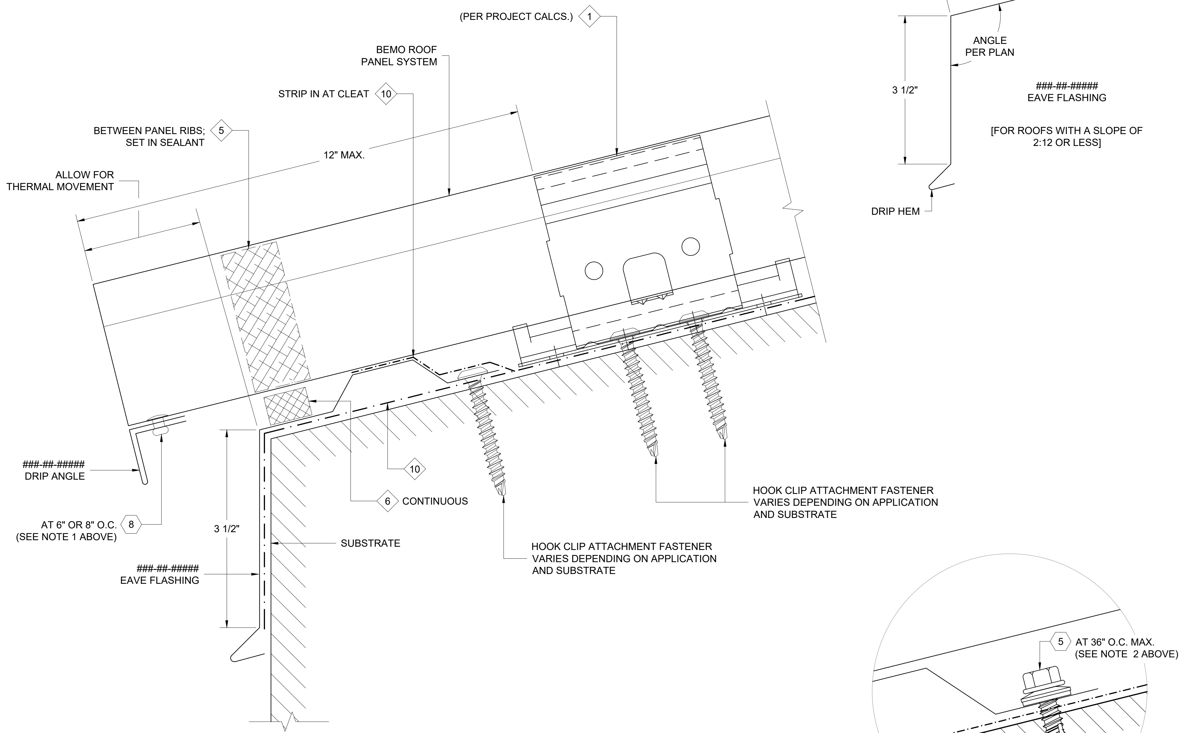
1 FLOATING EAVE DETAIL D1 REF. ARCH. DET. -
