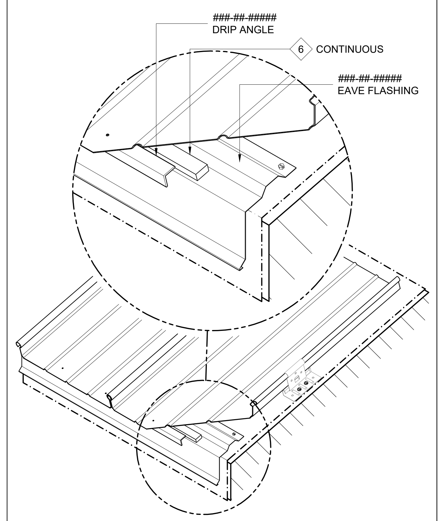
ISOMETRIC VIEW
