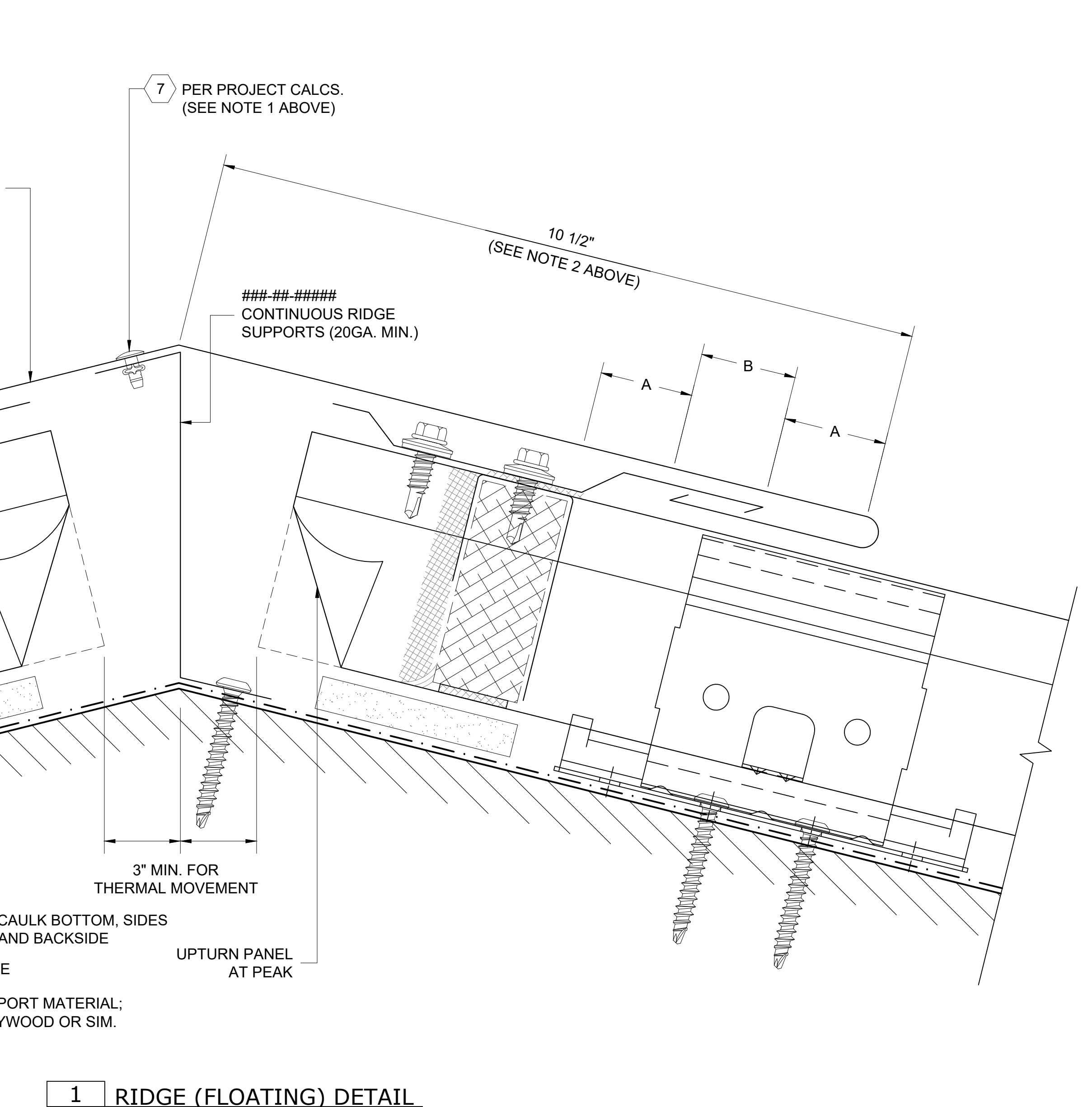
1 RIDGE (FLOATING) DETAIL D1 REF. ARCH. DET. -
