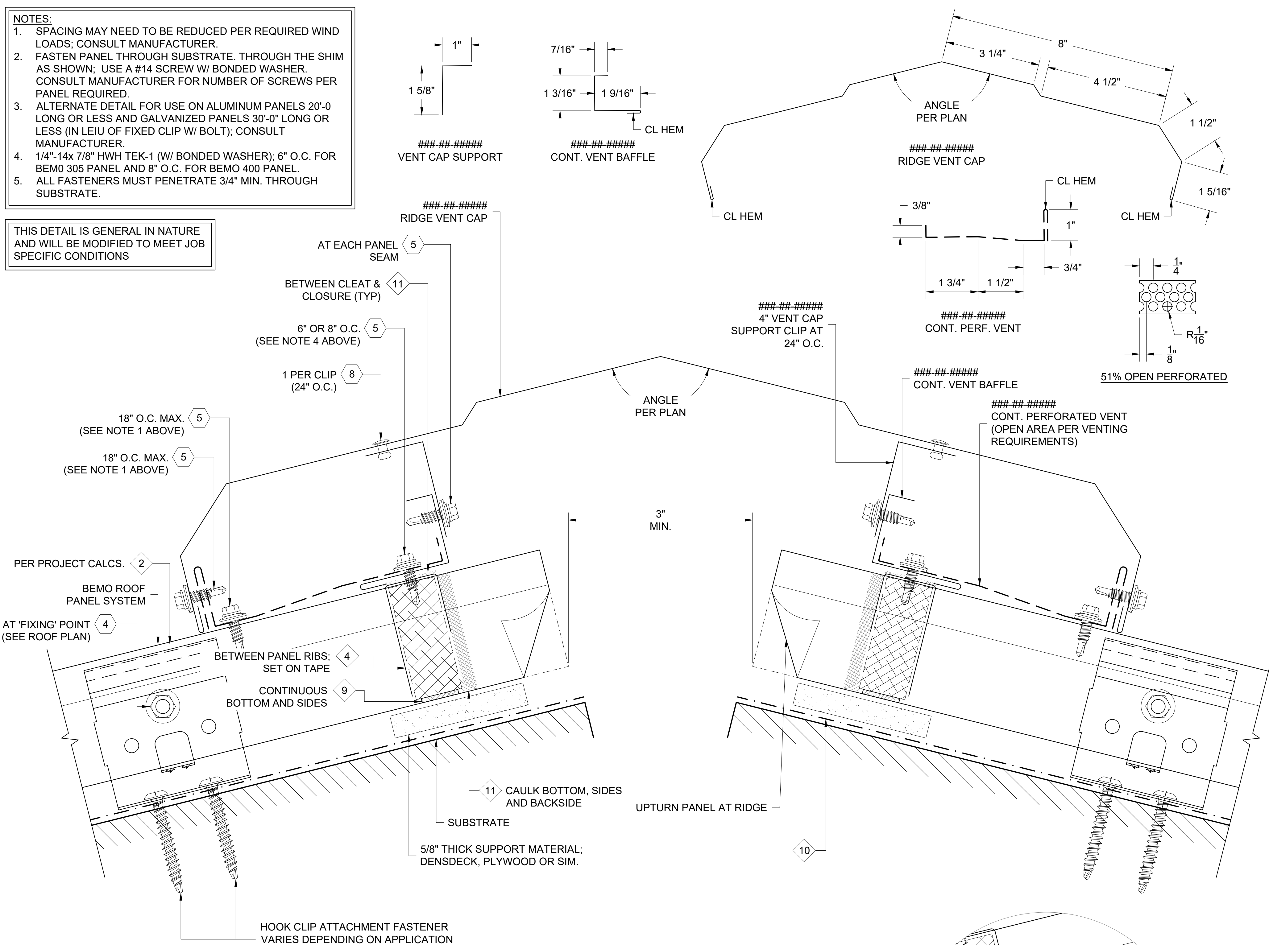
1 VENTED RIDGE (FIXED PANEL) DETAIL D1 REF. ARCH. DET. -
