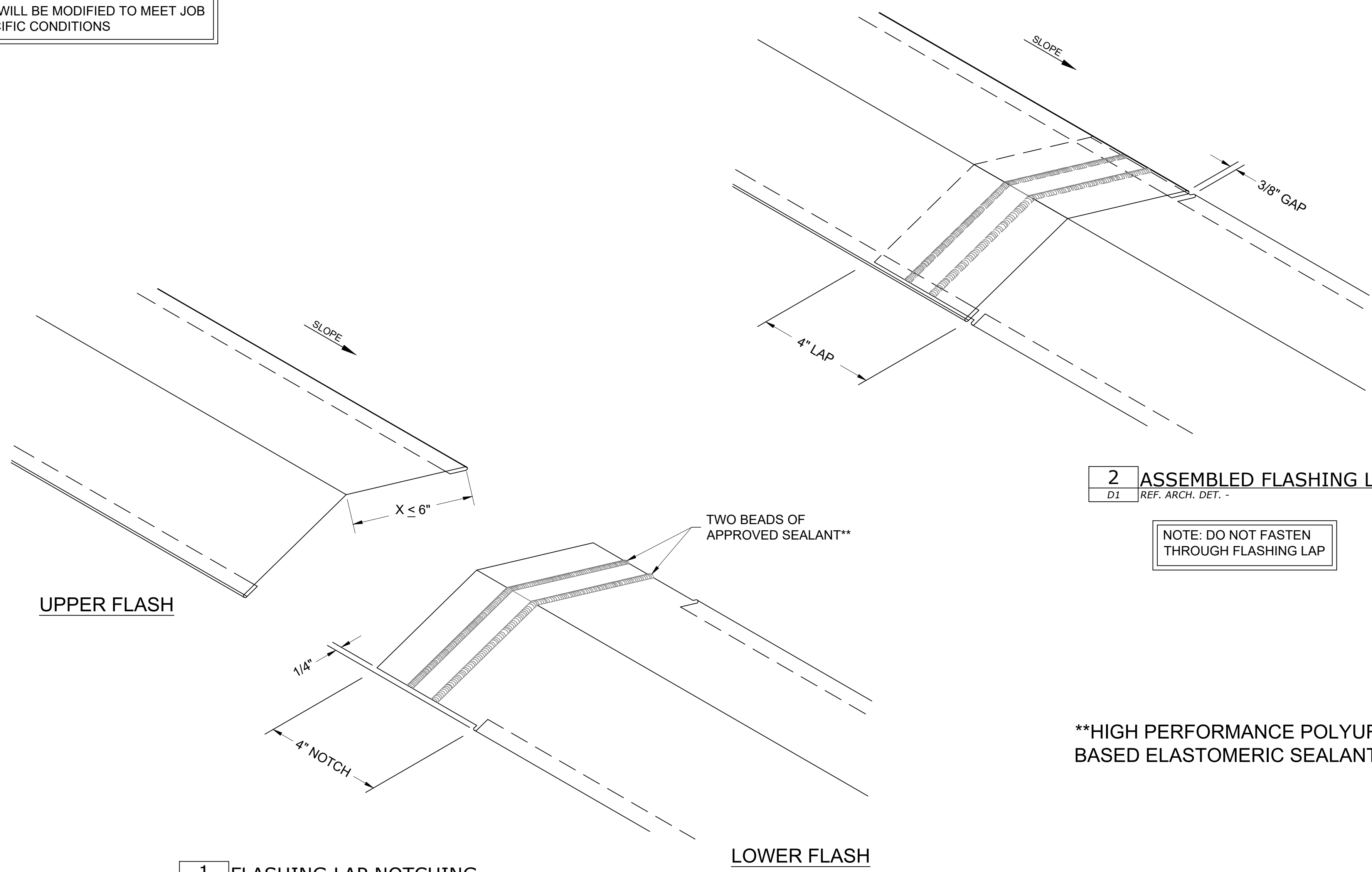
1 FLASHING LAP NOTCHING D1 REF. ARCH. DET. -
