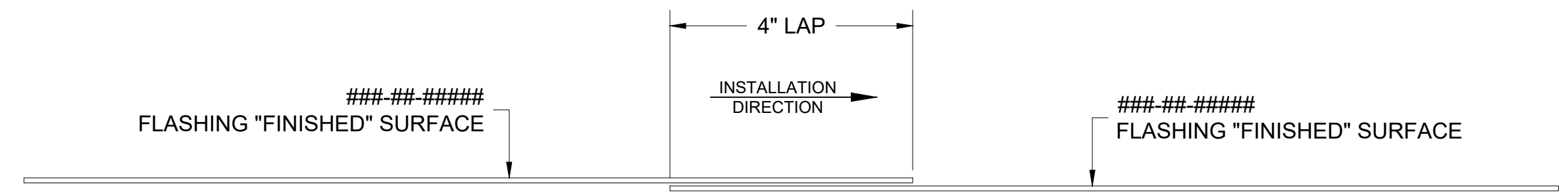
3 FLASHING LAP DETAIL D1 REF. ARCH. DET. -
