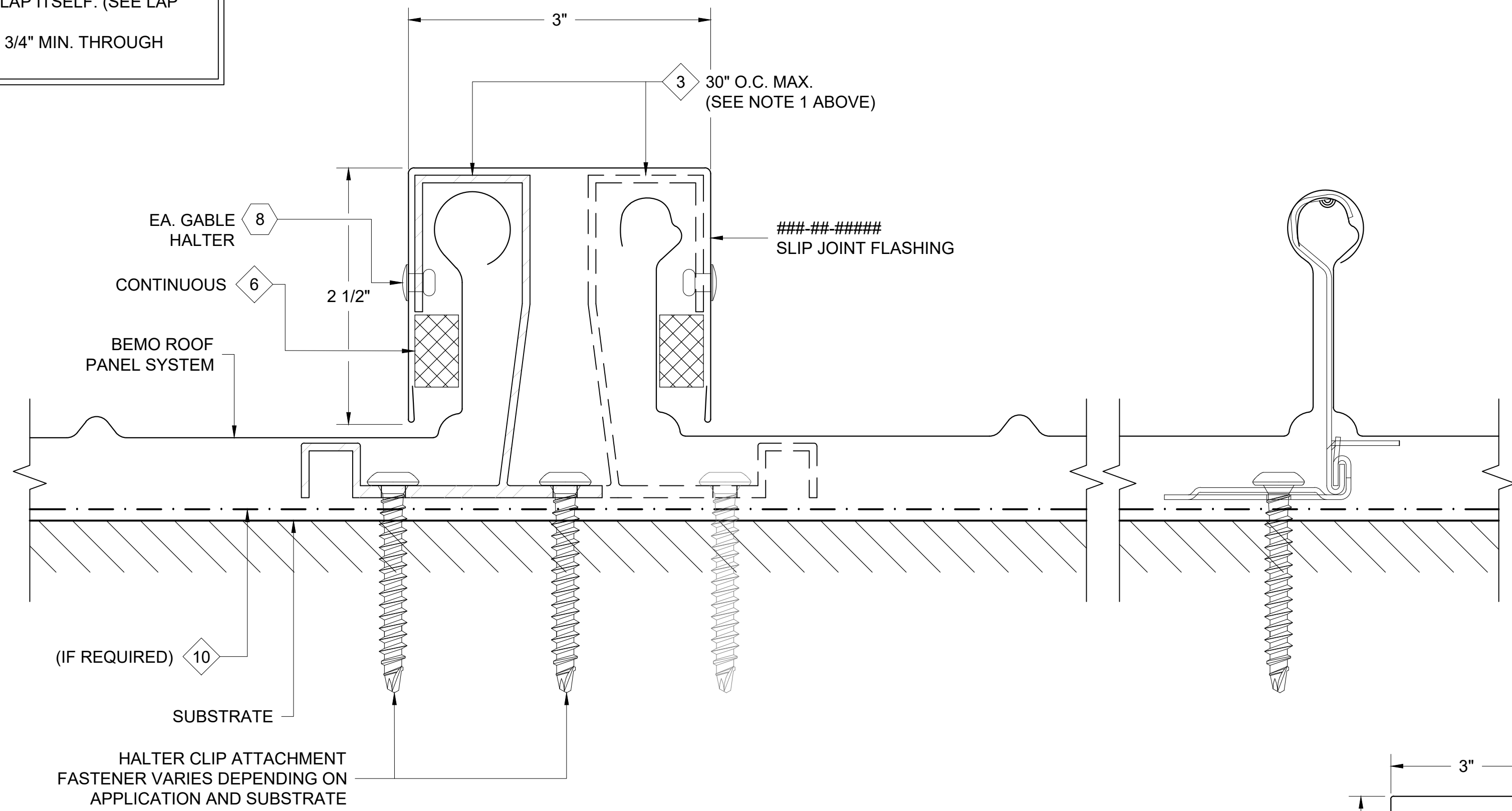
1 SLIP JOINT DETAIL D1 REF. ARCH. DET. -
