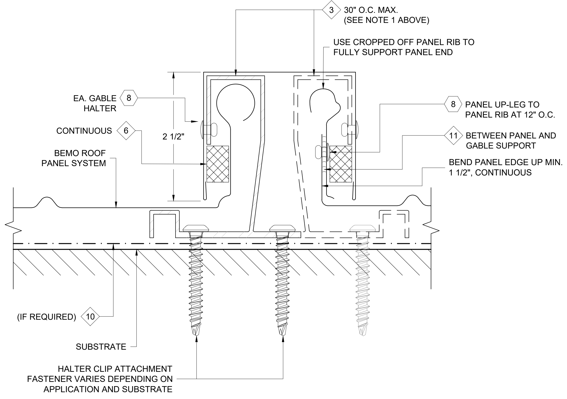
ALTERNATE DETAIL PANEL ENDS OFF MODULE
