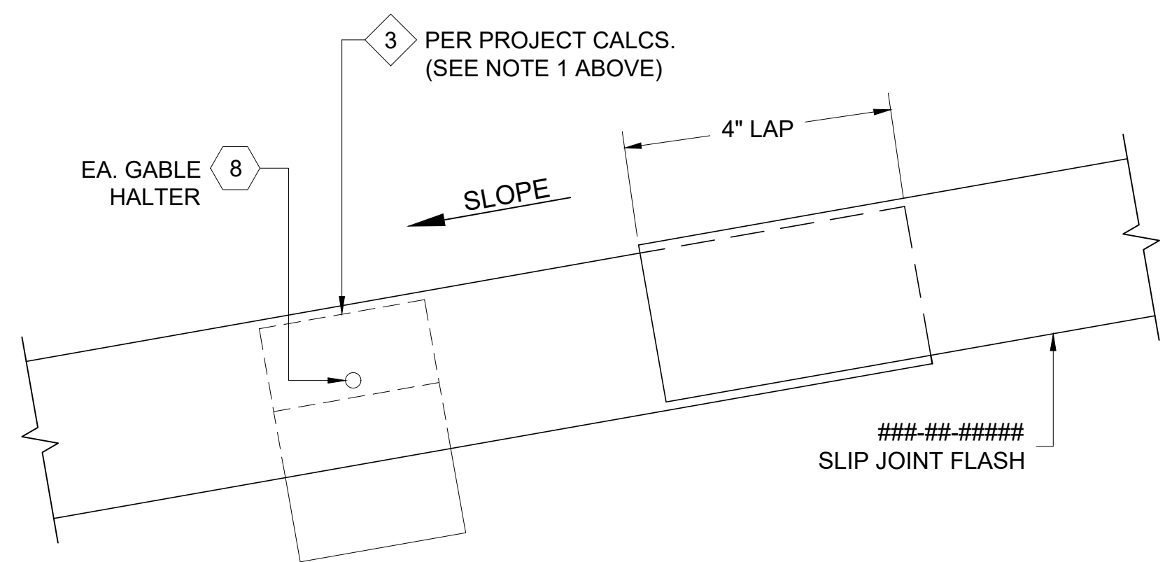
TYPICAL SLIP JOINT FLASHING LAP DETAIL
